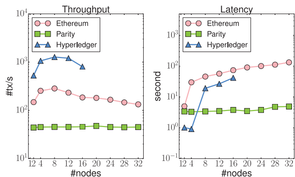
Fig. 8. Performance scalability (with the same number of clients and servers). The benchmark workload is YCSB. The scalability against Smallbank is similar, except that Hyperledger fails beyond eight nodes instead of 16.
